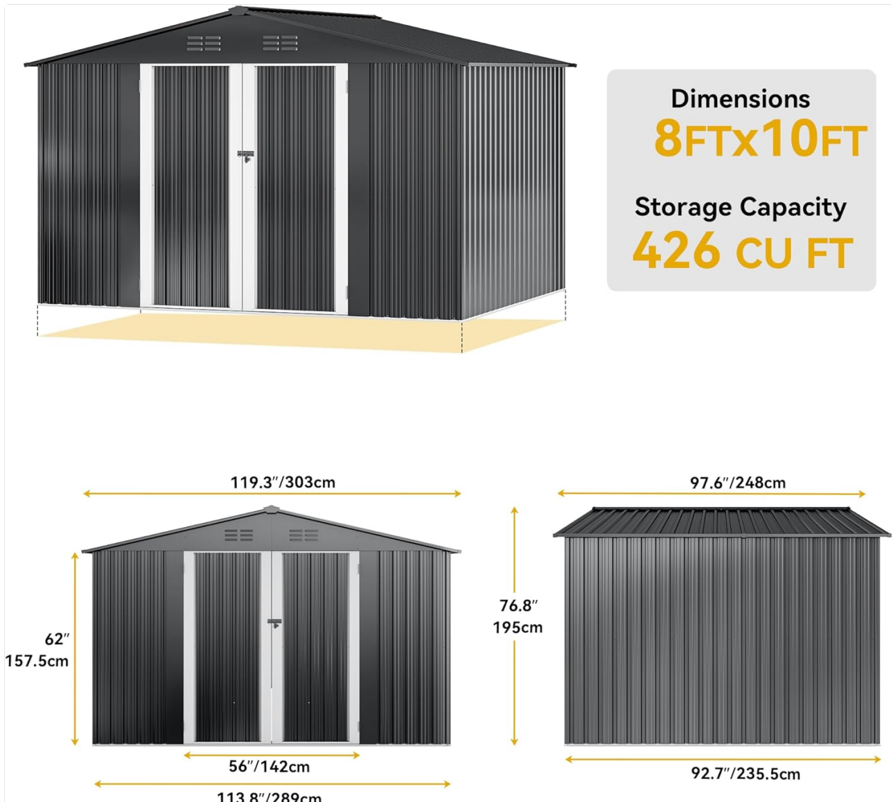
Image 5.1: Shed dimensions, useful for planning and assembly.
