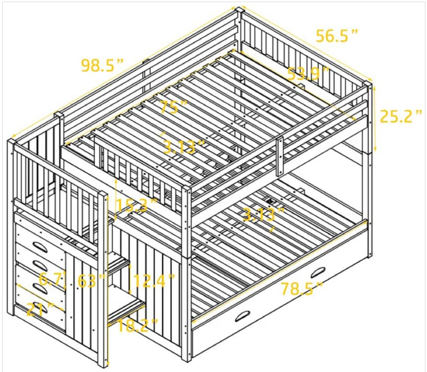
Image: A detailed dimension diagram of the bunk bed, illustrating the overall length, width, height, and specific measurements for each section, including the upper and lower bunks, staircase, and trundle.
