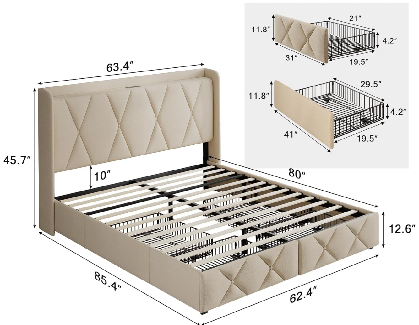
Figure 8.1: Detailed dimensions of the GalnFu Queen Bed Frame.
