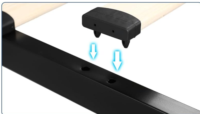
Figure 4.1: Details of the sturdy metal frame, noise-free EVA silent strip, and embedded slat design for easy assembly.
