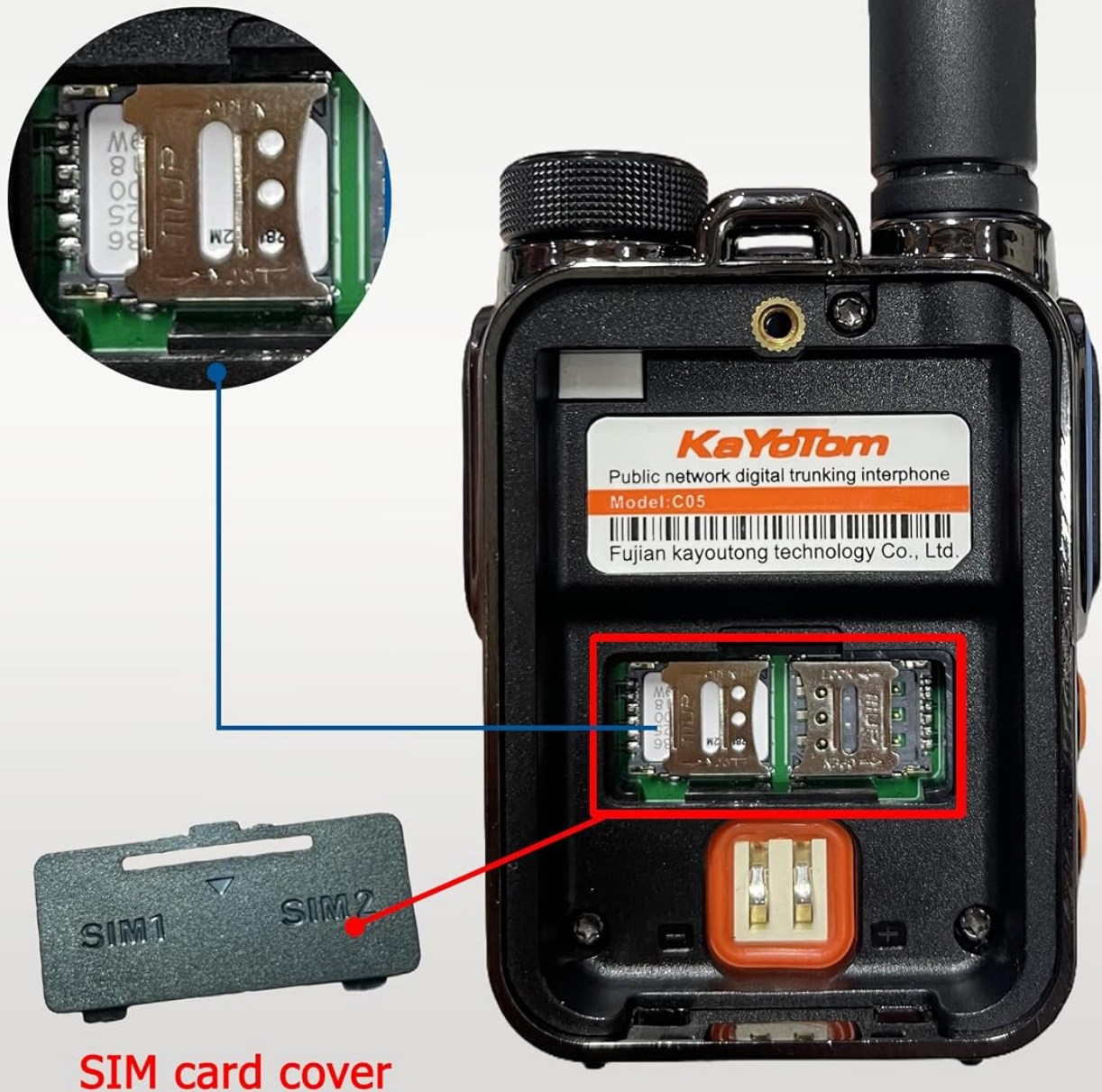
Figure 5: SIM Card Slot Location
