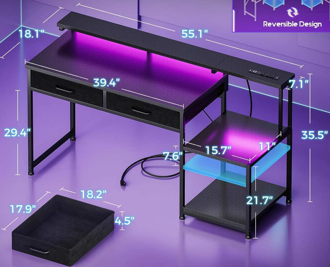
Image 4.1: Desk dimensions and illustration of the reversible side shelf design.
