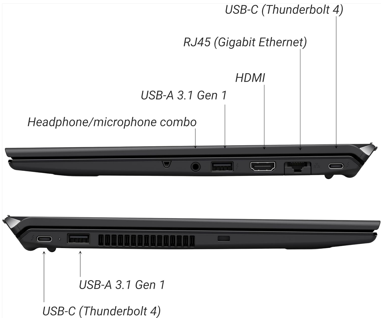
Figure 2: Port layout of the VAIO SX-R Laptop. The left side includes a headphone/microphone combo jack, USB-A 3.1 Gen 1, HDMI, RJ45 (Gigabit Ethernet), and USB-C (Thunderbolt 4). The right side features another USB-C (Thunderbolt 4) and USB-A 3.1 Gen 1 port.
