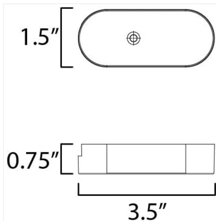
Figure 2: Dimensional drawing of the ETMSC04-WT driver. The driver measures 3.5 inches in length, 1.5 inches in width, and 0.75 inches in height, providing precise measurements for installation planning.
