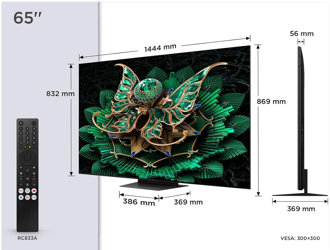
Image: Detailed dimensions of the TCL 65C7K TV and its remote control, useful for planning installation.
