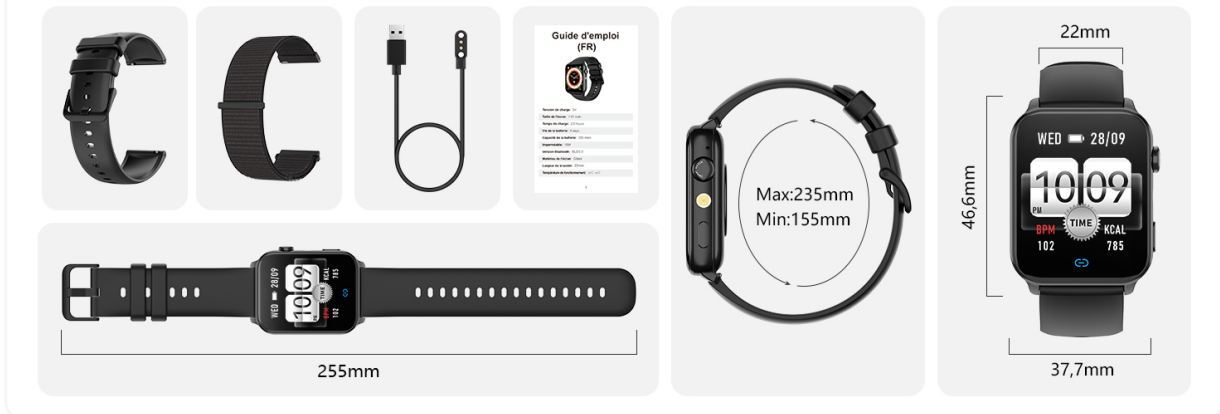
Image: Detailed product dimensions of the Blackview R30max smartwatch.
