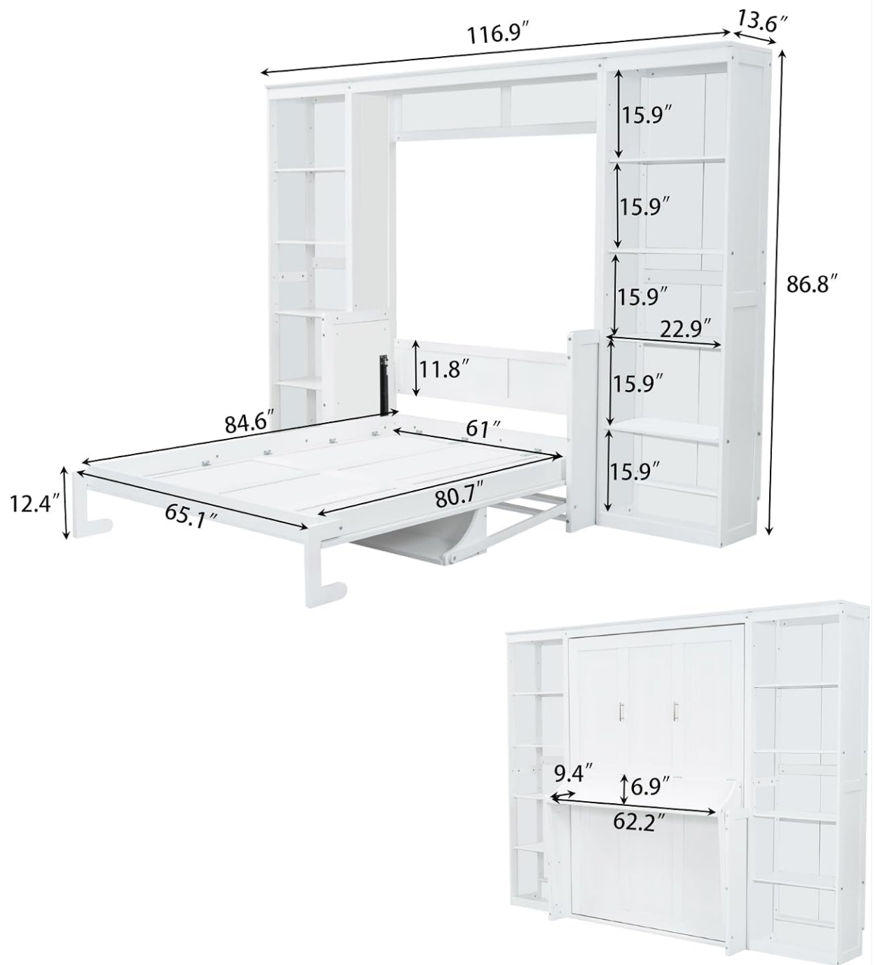
Figure 3.1: Dimensional diagram of the Murphy bed, illustrating key measurements for planning your space.
