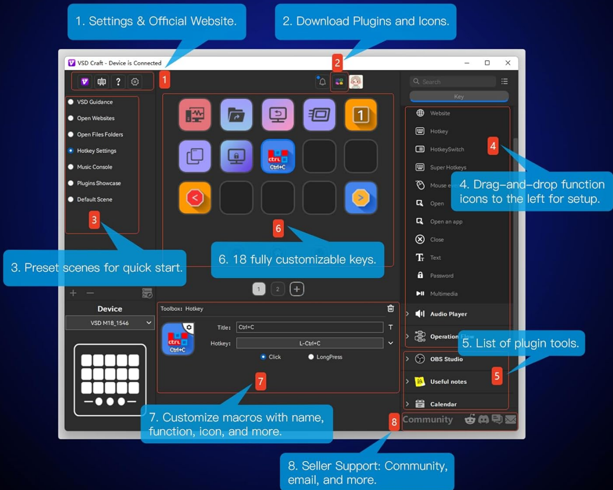
Image: A screenshot of the VSD Craft software interface, demonstrating how to drag and drop actions onto the 18 customizable keys and configure settings.
