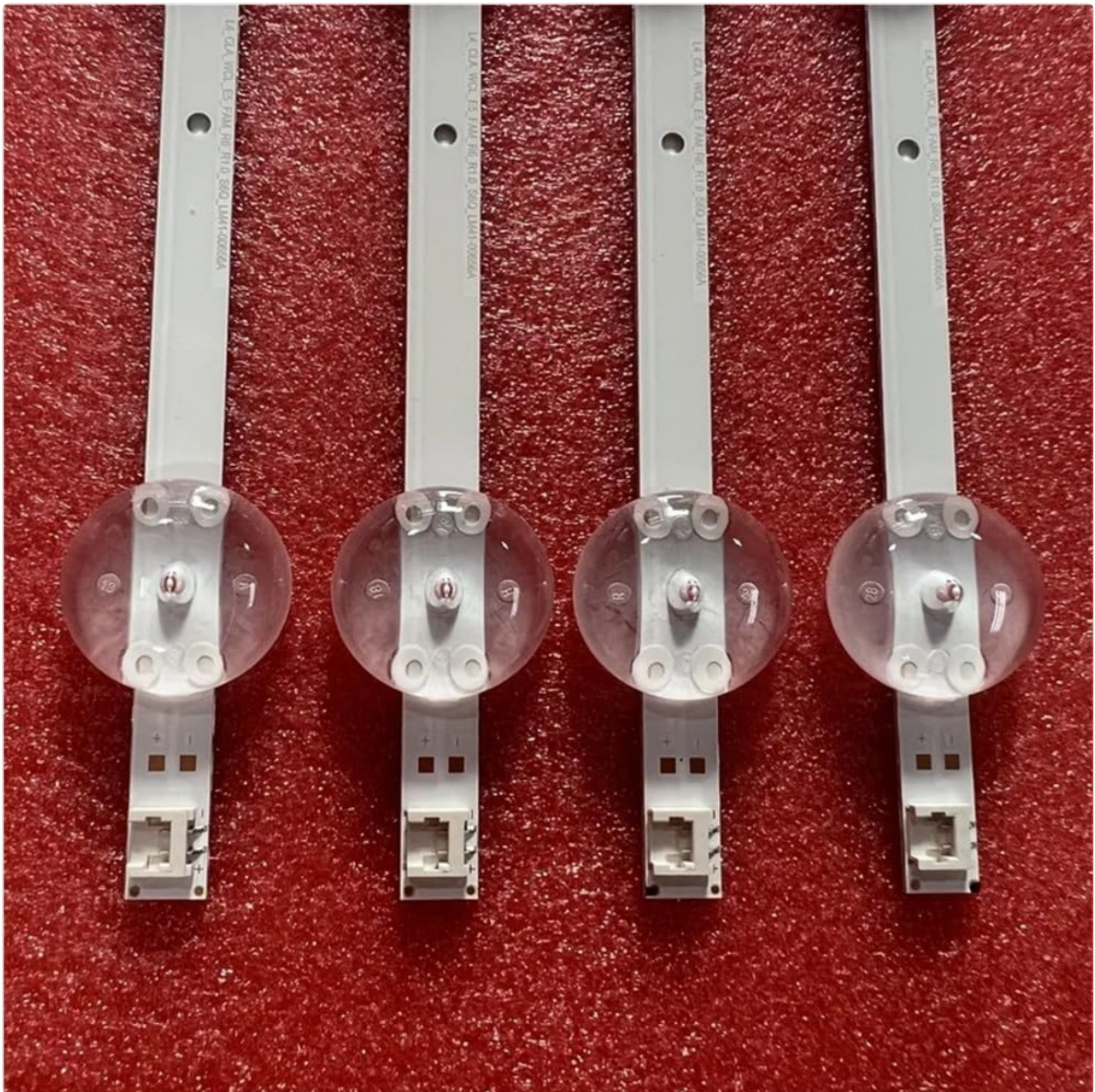
Figure 4.1: Detail of LED strip connectors.
