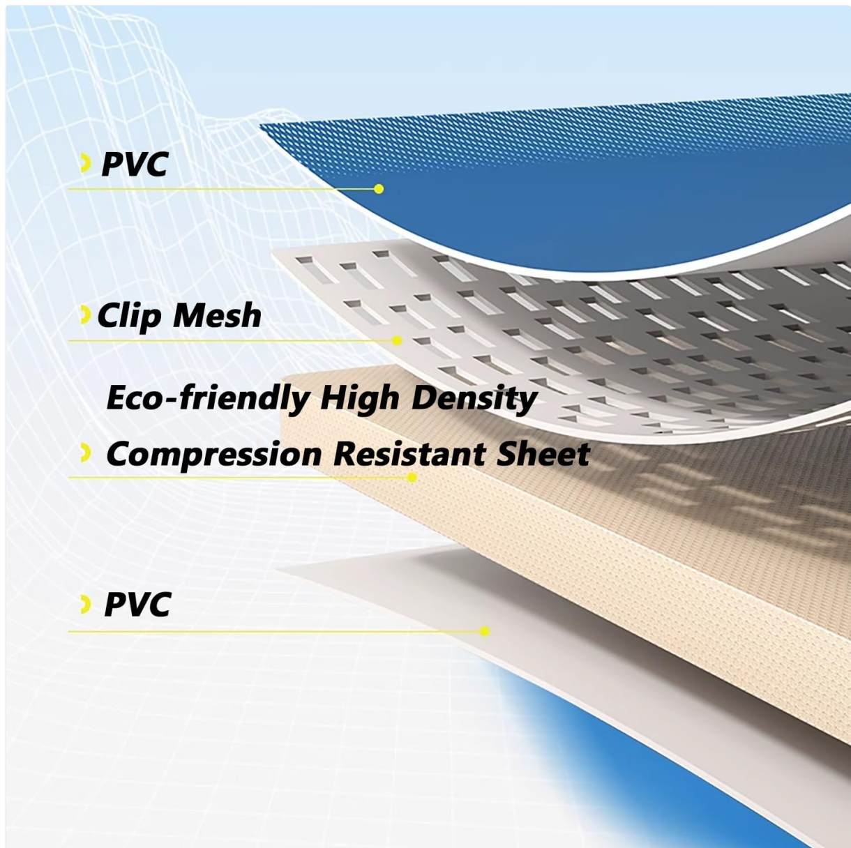
Figure 6.1: Multi-layer PVC material construction for durability.
