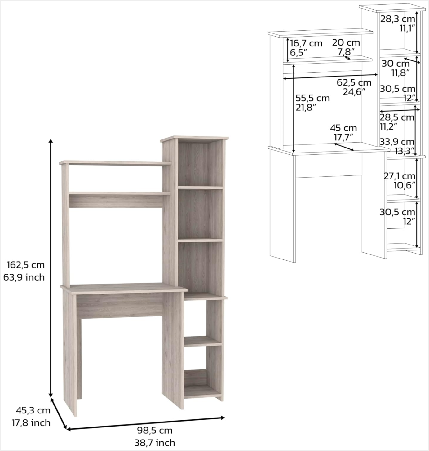
Image 4: A technical diagram illustrating the precise dimensions of the desk, including overall height, width, and depth, as well as individual measurements for the hutch shelves and side bookcase compartments. Measurements are provided in both inches and centimeters.
