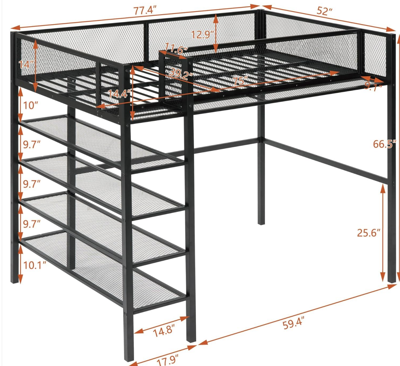
Image: A detailed diagram showing the overall dimensions of the loft bed in inches, including height, length, width, and shelf dimensions, crucial for planning placement and assembly.
