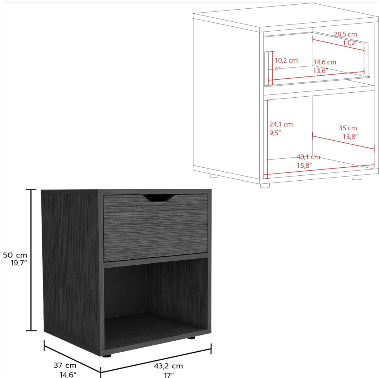
Figure 6.1: Dimensional diagram of the nightstand, illustrating its height, width, and depth, along with internal drawer and shelf measurements.
