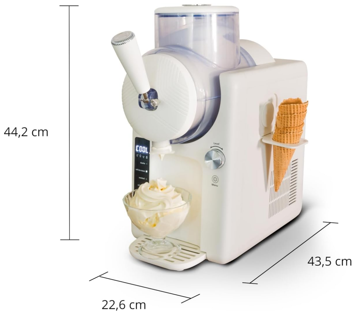
Image: The Unold 48950 machine with overlaid dimensions: 44.2 cm height, 43.5 cm depth, and 22.6 cm width, providing a clear understanding of its physical size.
