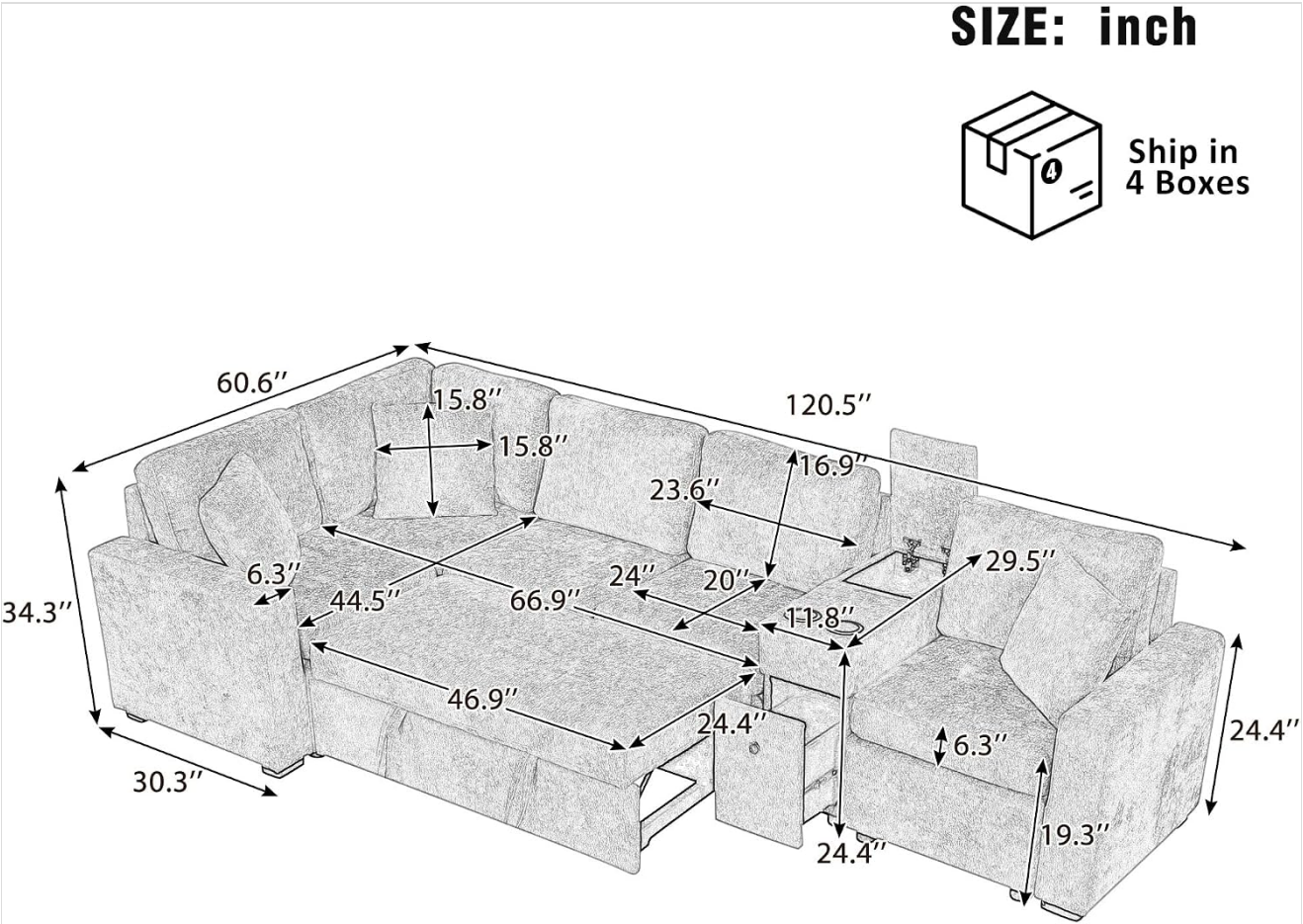
Image 8.1: Detailed product dimensions.
