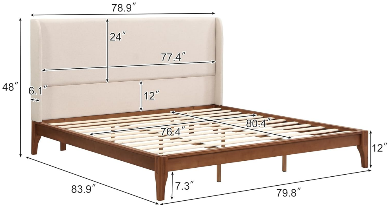
Figure 1: Detailed dimensions of the Polibi King Size Platform Bed, including overall length, width, headboard height, and under-bed clearance.
