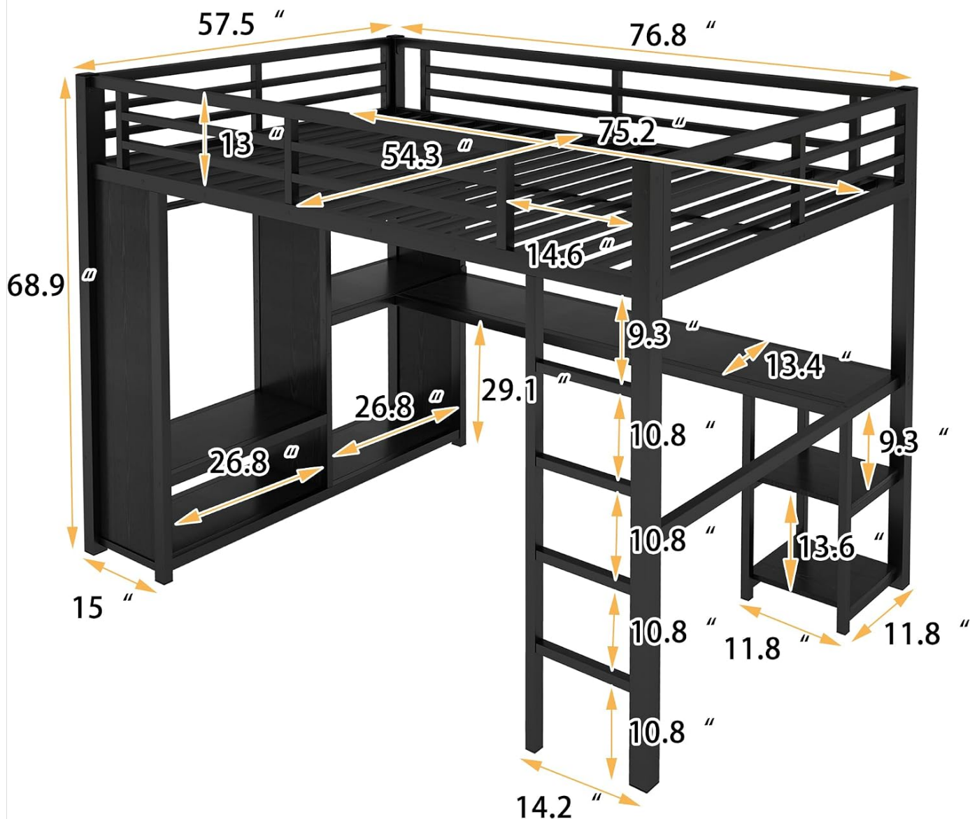
Figure 1: Overall dimensions of the loft bed structure.
