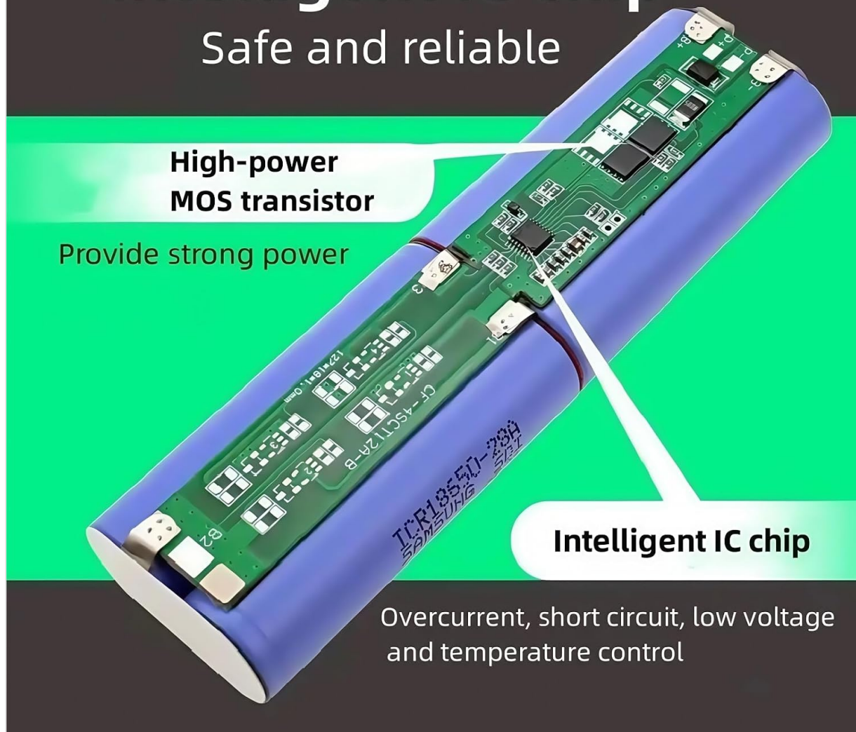
Figure 1: Internal components of the battery, highlighting the intelligent IC chip for overcurrent, short-circuit, low voltage, and temperature control, and a high-power MOS transistor for strong power delivery.
