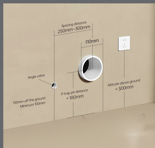
Figure 3: Diagram illustrating rear outlet plumbing requirements.
