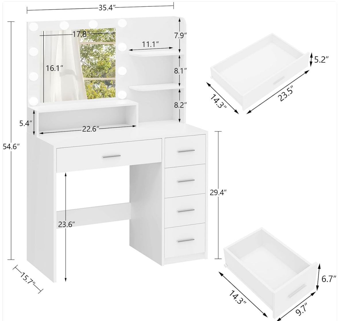
Figure 3.1: Vanity Desk Dimensions and Key Components
