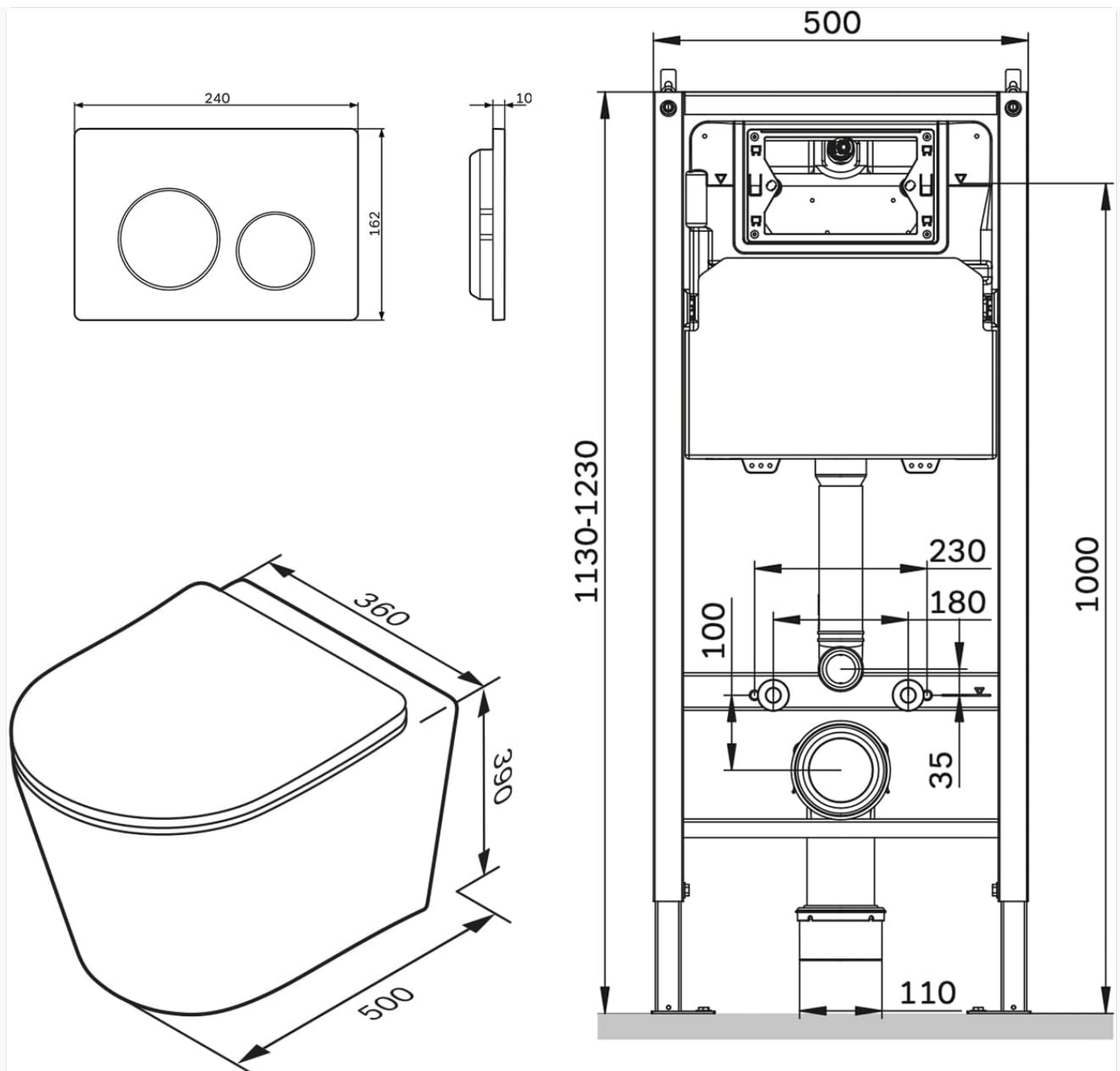
Image: Technical drawing illustrating the overall dimensions of the wall element, flush plate, and the installed WC.
