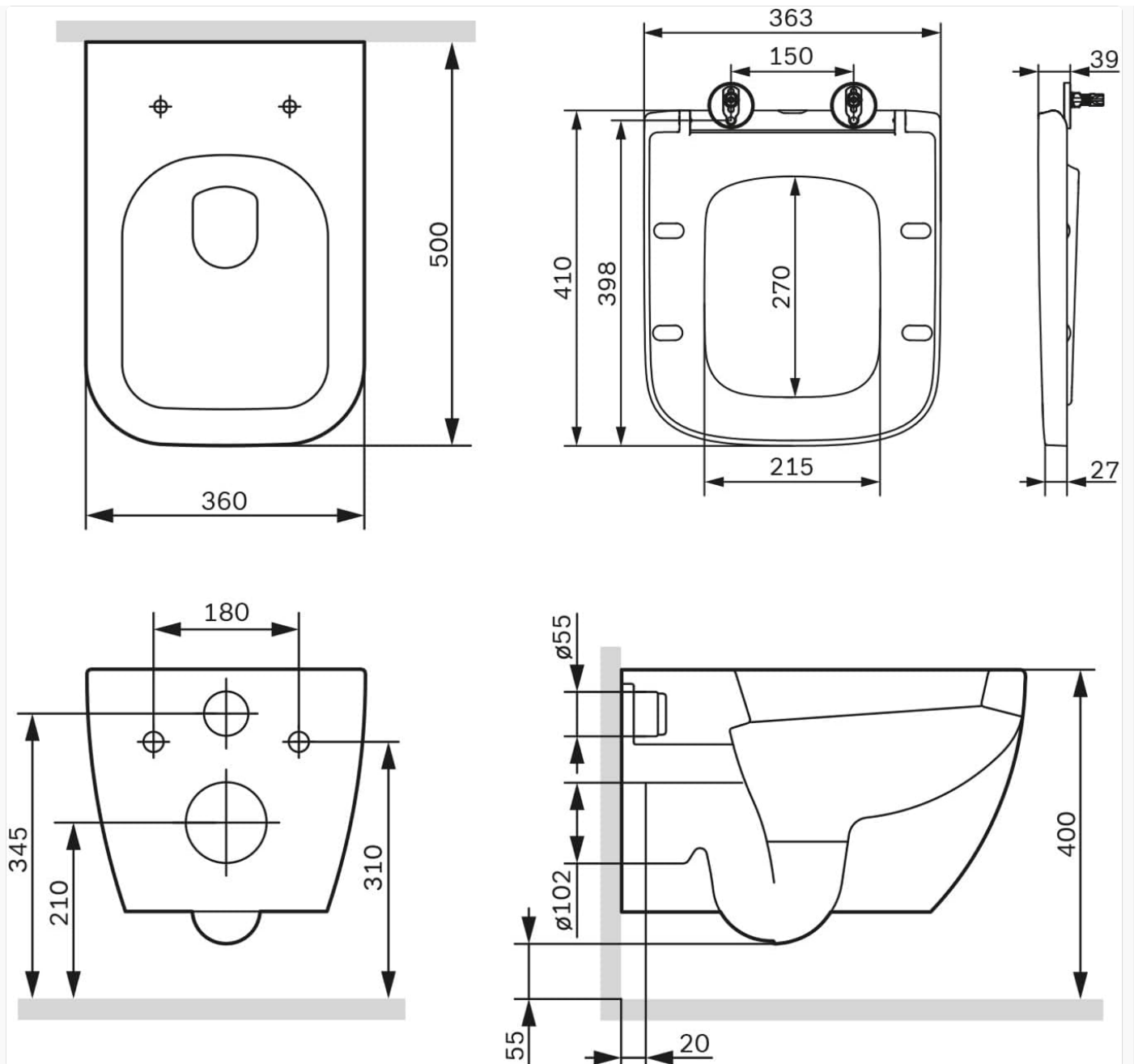
Image: Technical drawing detailing the dimensions of the wall-hung WC bowl and seat.
