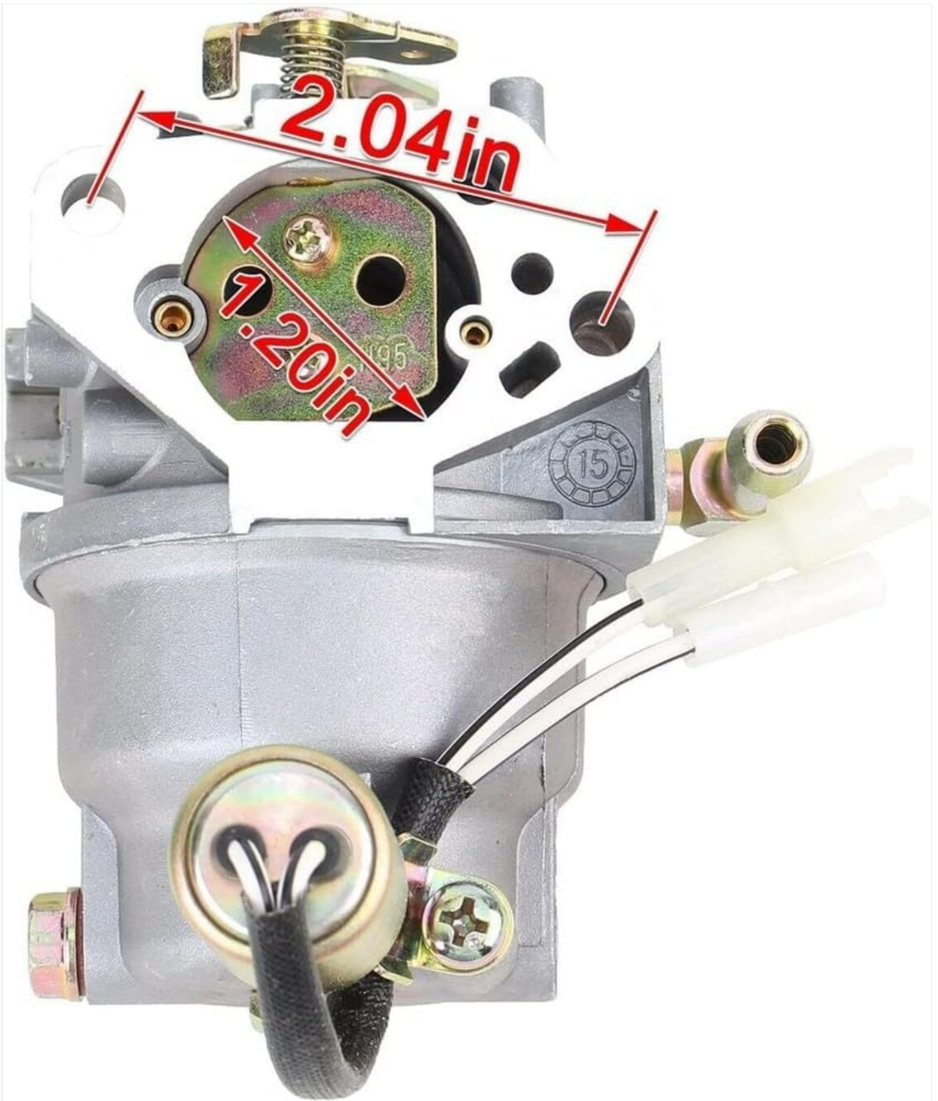
Figure 4: Side view of the carburetor with approximate dimensions indicated (e.g., 2.04in and 1.20in). These provide further detail for fitment verification.
