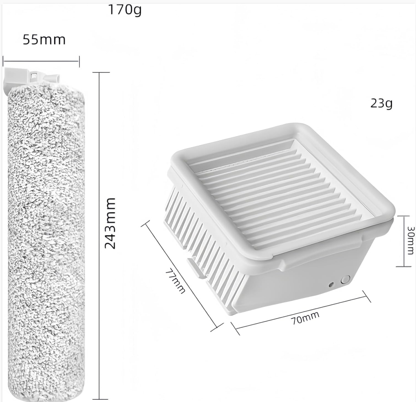
Image 4: Dimensions of the roller brush (243mm length, 55mm width) and filter (77mm length, 70mm width, 30mm height).
