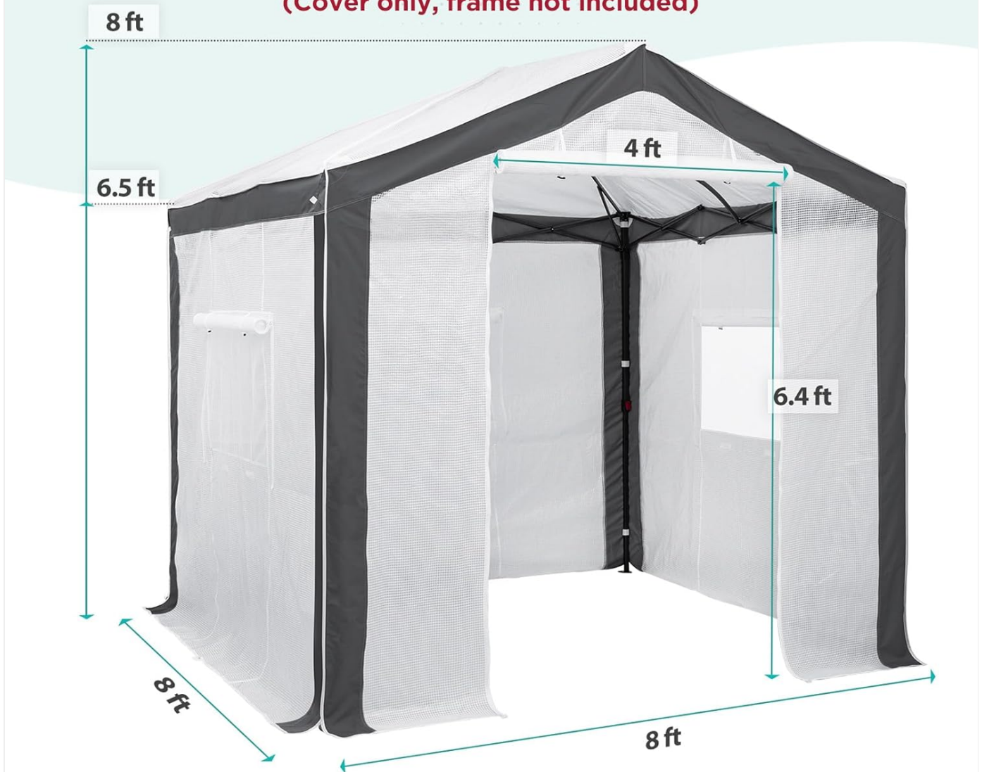
Figure 6.1: Overall dimensions of the 8'x 8' replacement cover (frame not included).
