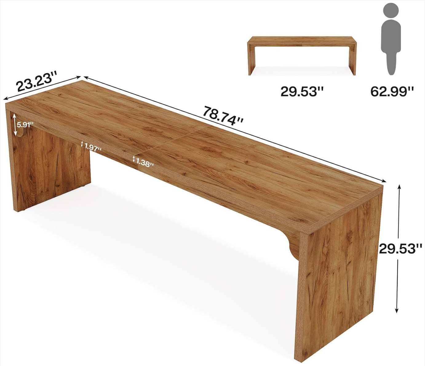
Image: Detailed dimensions of the desk, including width, depth, and height, for accurate planning and placement.
