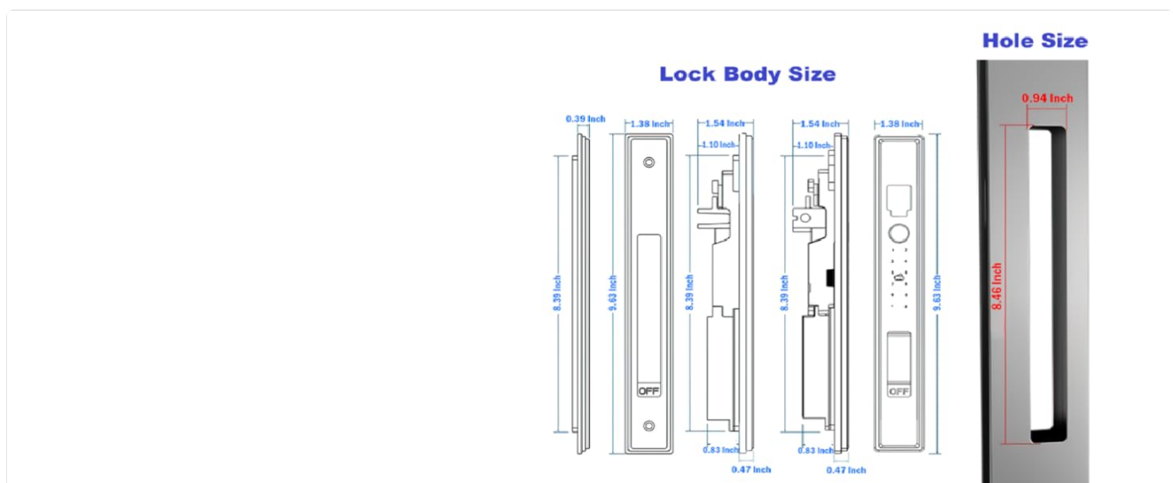
Image: Technical drawing detailing the lock body dimensions and the necessary door hole size for proper installation.
