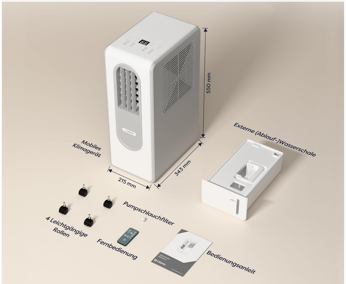
Figure 3.1: Contents of the CIARRA Mobile Air Conditioner package.
