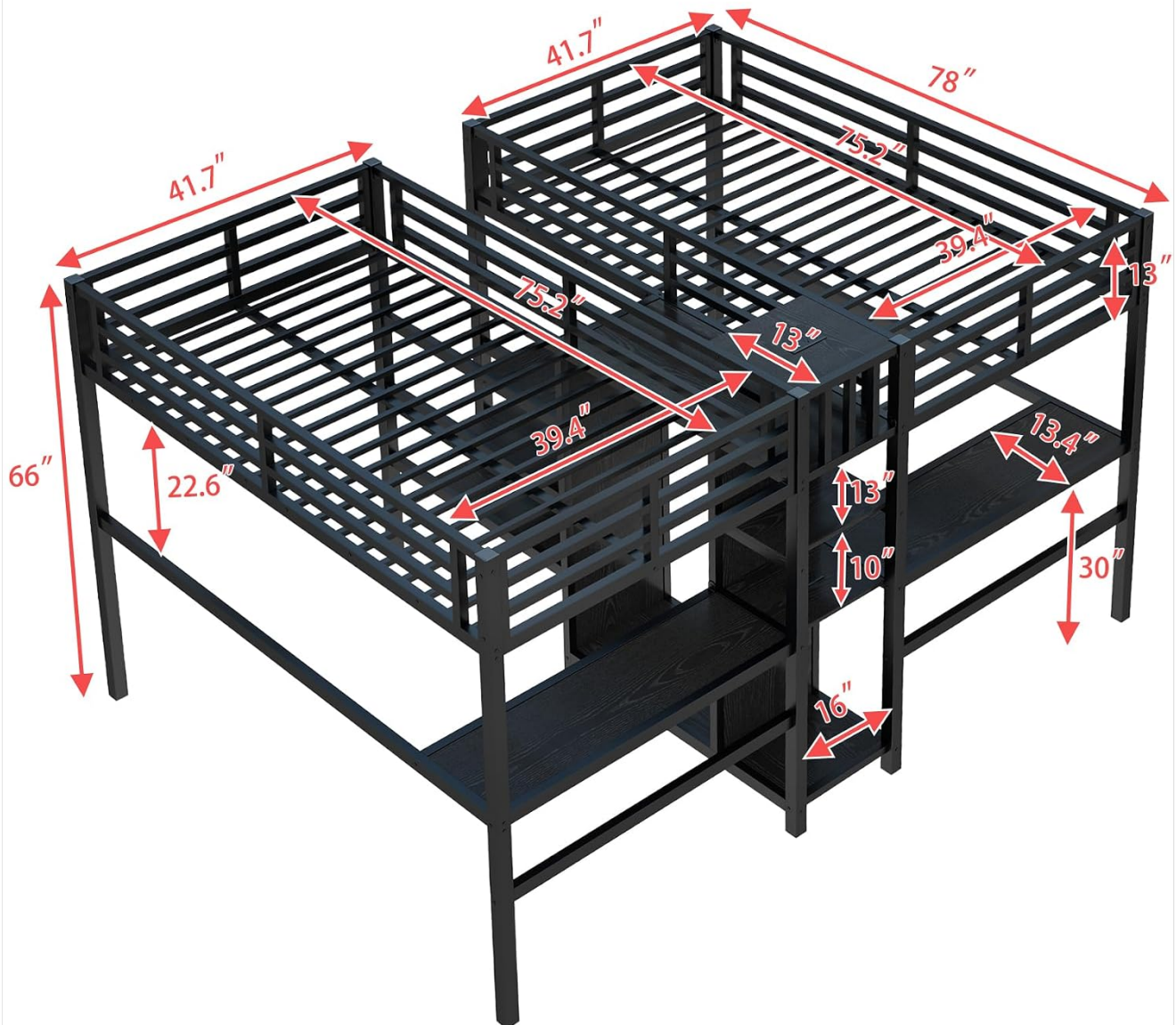
Image 8.1: Detailed dimensions of the loft bed in inches, illustrating length, width, and height measurements for various components.
