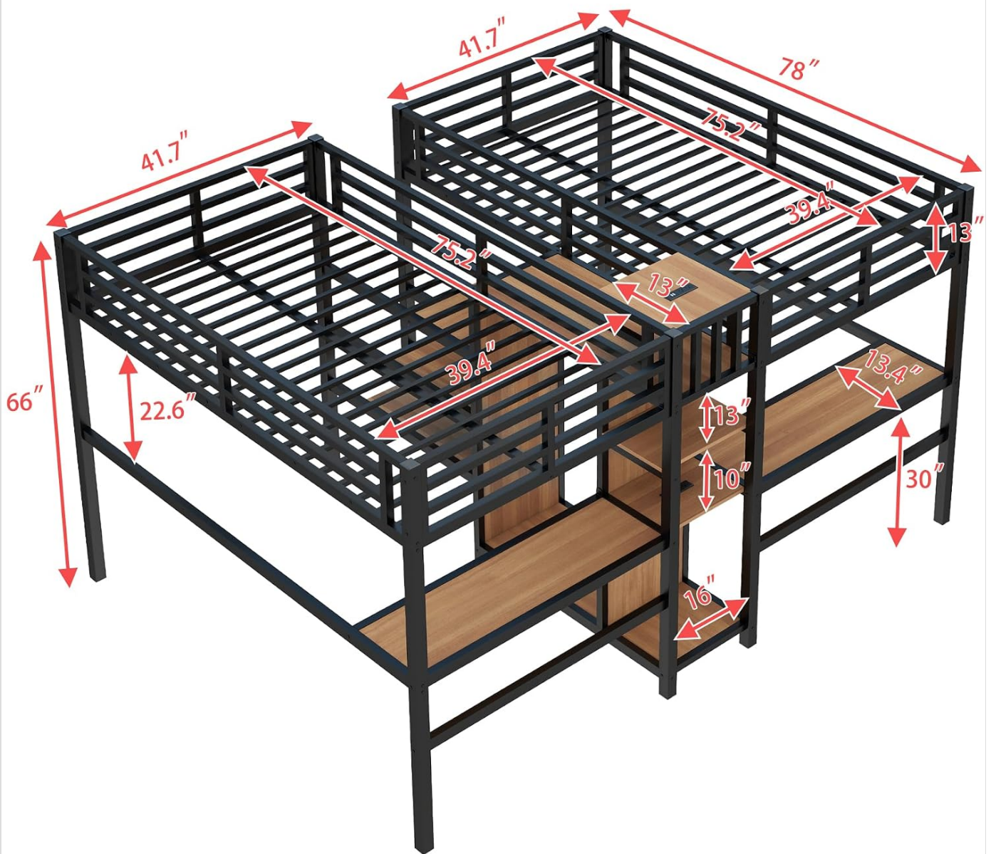
Figure 1: Overall dimensions of the loft bed. The bed measures 99.4"L x 78"W x 66"H.
