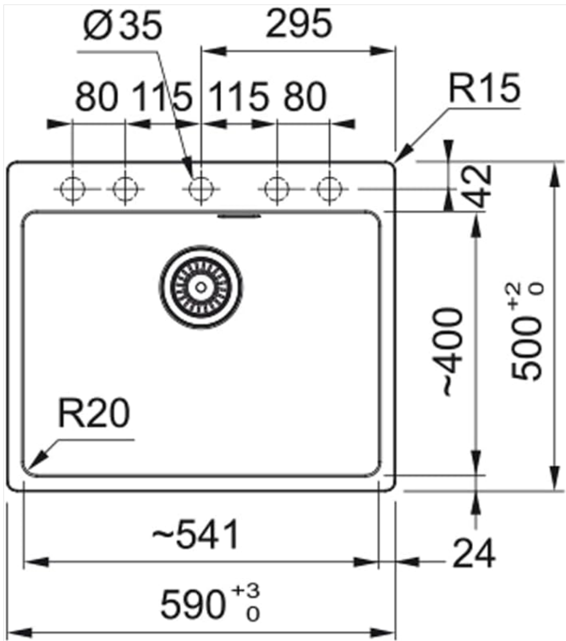
Image: Technical drawing with dimensions for installation.
