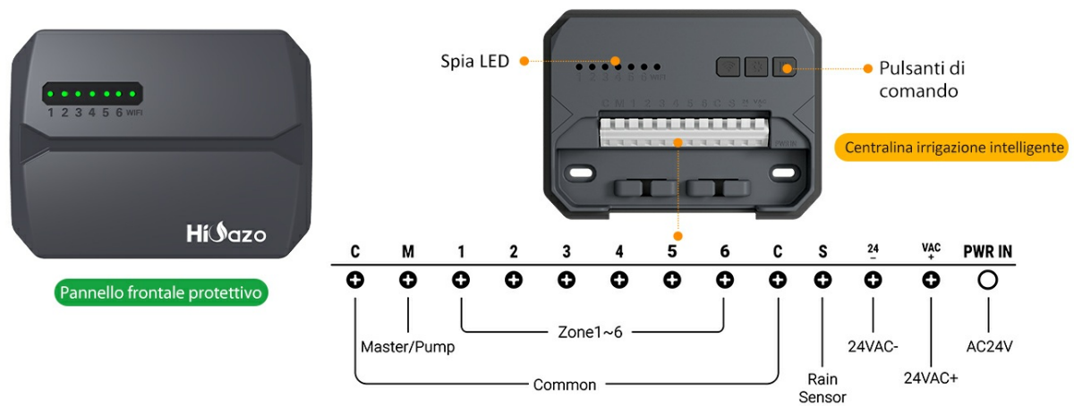
Figure 2: Wiring diagram and component layout of the HiOazo HSC-600W controller. This diagram illustrates the connection points for the master valve/pump, individual zone valves (1-6), common wire, rain sensor, and 24VAC power input. LED indicators and control buttons are also shown.
