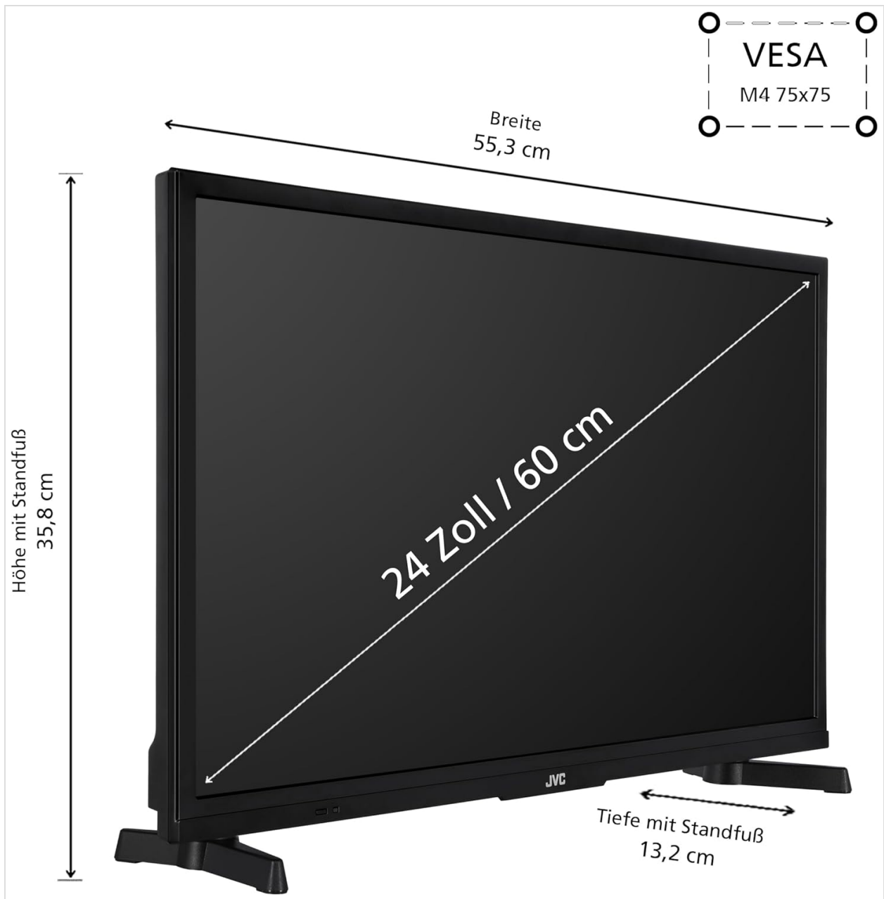
Image 4.1: Dimensions of the JVC LT-24VAH3455 TV. Height with stand: 35.8 cm, Width: 55.3 cm, Depth with stand: 13.2 cm. VESA mount: M4 75x75.
