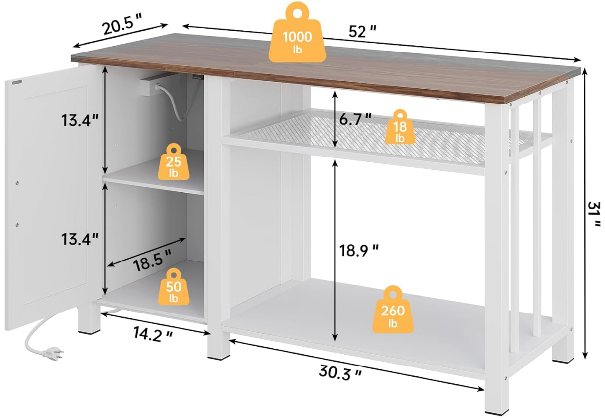
Image: Detailed product dimensions and weight distribution for the stand.
