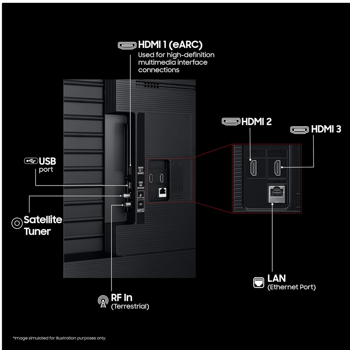
Image: Rear panel connections, illustrating HDMI (eARC), USB, Satellite Tuner, RF In (Terrestrial), and LAN (Ethernet Port).
