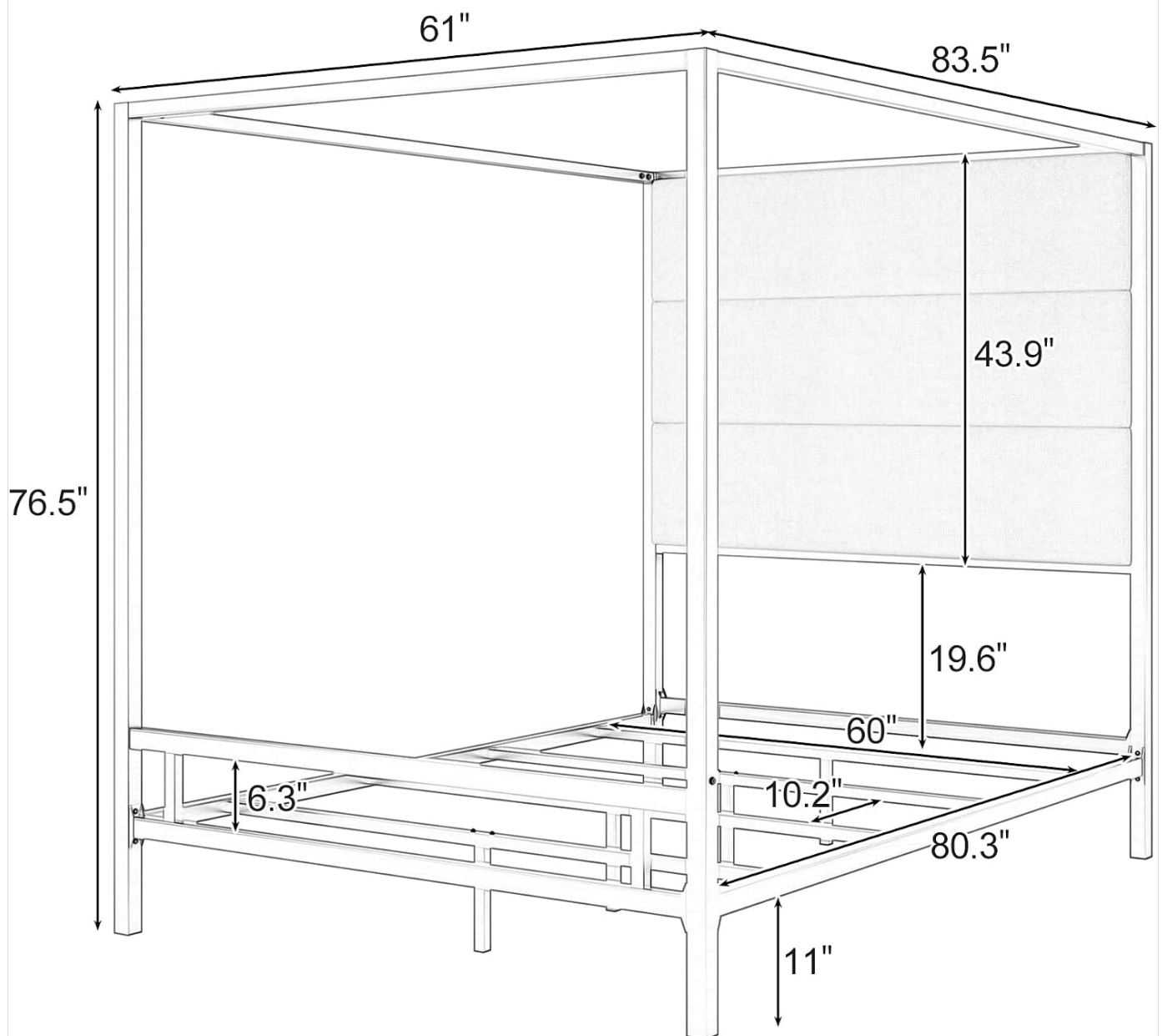
Figure 1: Queen size bed dimensions. The bed measures 83.5 inches in length, 61 inches in width, and 76.5 inches in height. Key measurements for the frame and headboard are also indicated.
