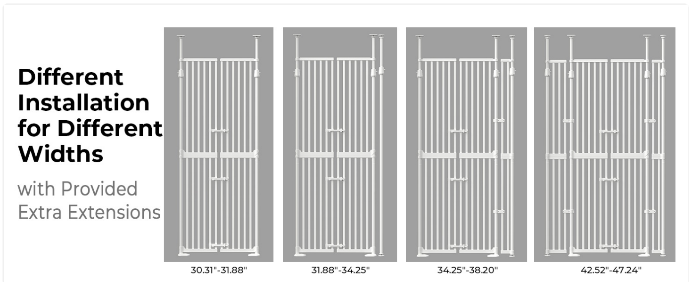
Figure 3: Different Installation for Different Widths. This diagram shows how to use extension panels to adapt the gate to various opening sizes, from 30.31"-31.88" to 42.52"-47.24".
