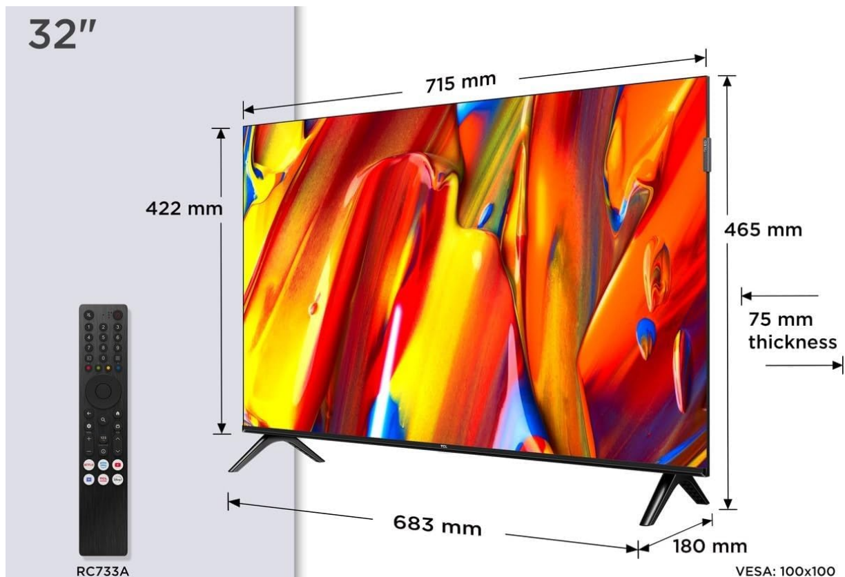
Image: Diagram showing the dimensions of the TCL 32V5C TV and the included remote control (RC733A).
