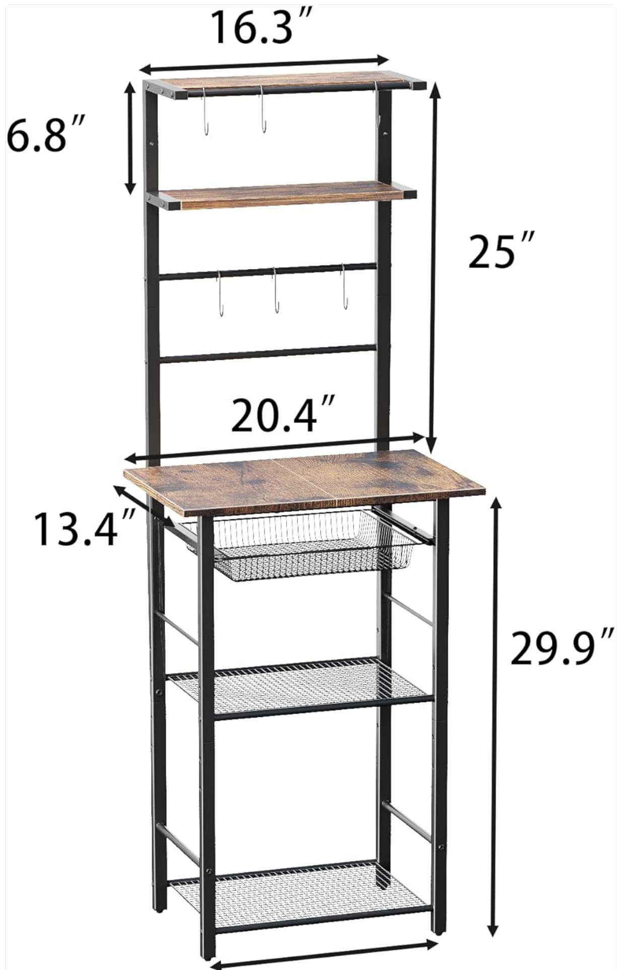
Figure 2: Dimensional diagram of the rack, illustrating key measurements for various sections and shelves. This helps in identifying parts during assembly.
