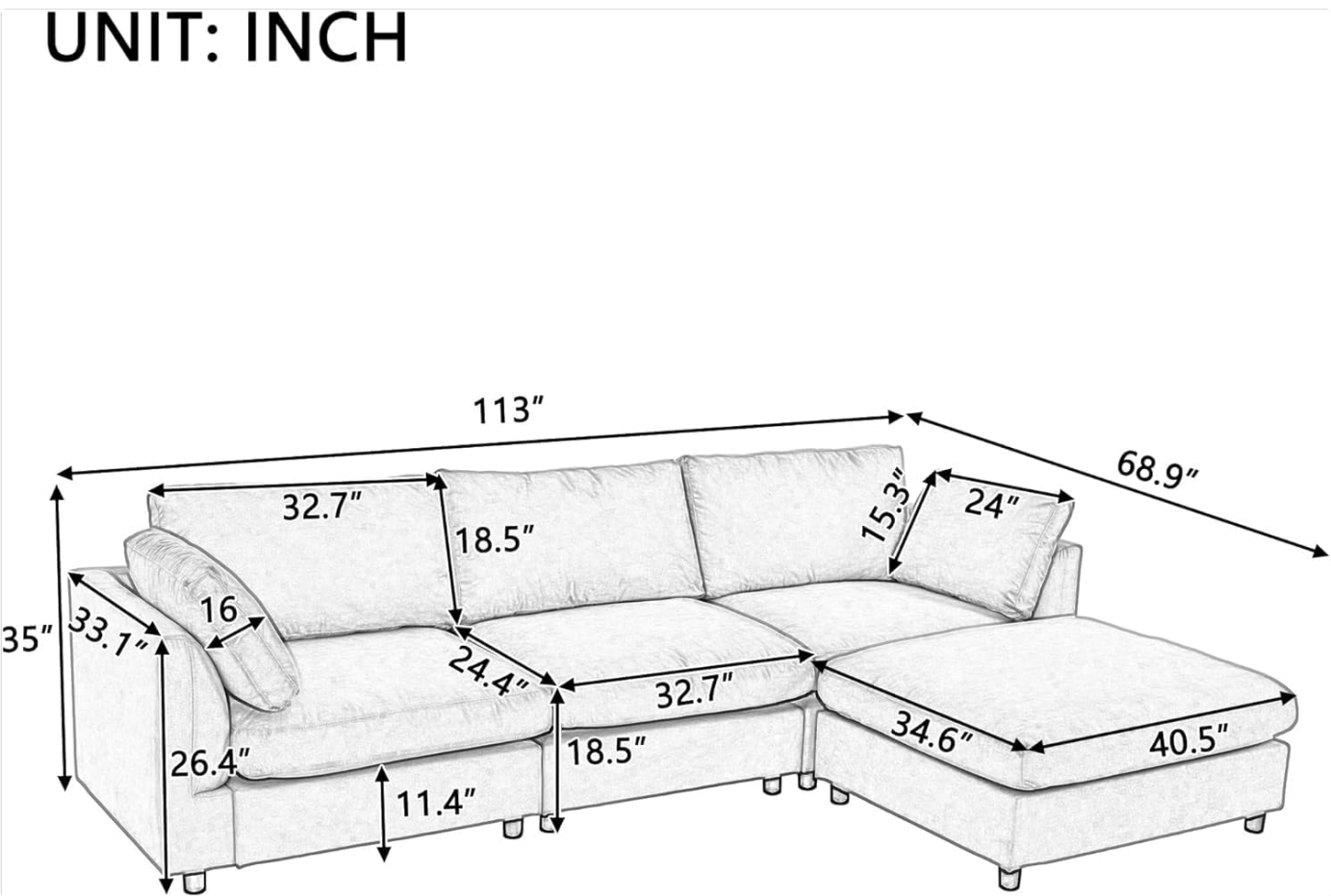
Image: Dimensional diagram of the sofa, illustrating overall length, depth, and height, as well as individual cushion and armrest measurements.
