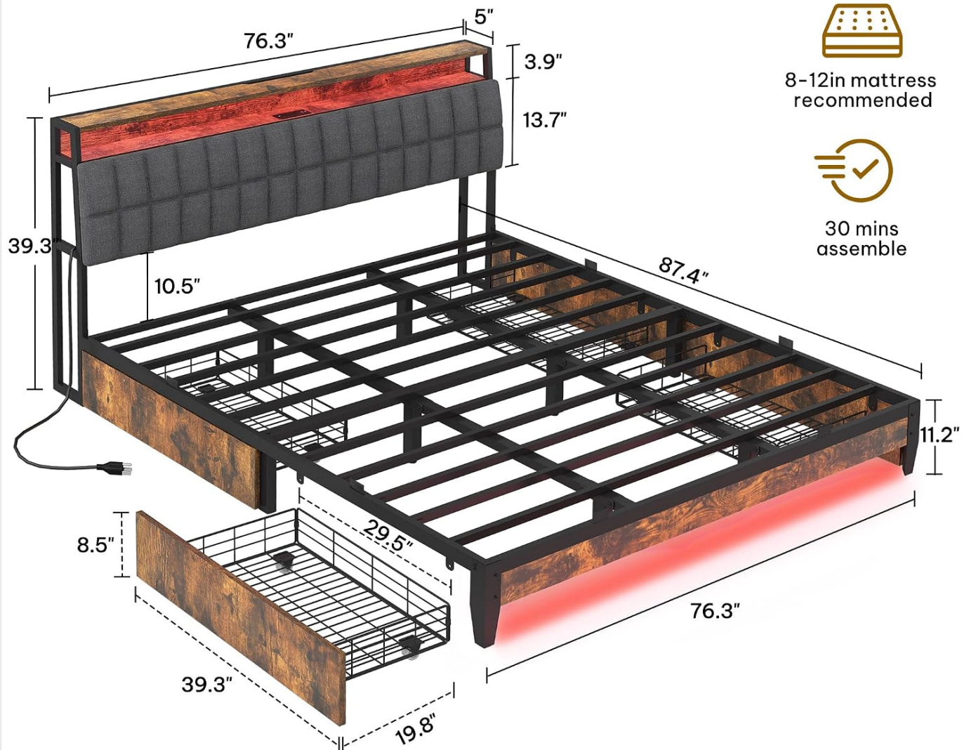
Figure 3.1: Product dimensions and key components. Recommended mattress thickness is 8-12 inches.
