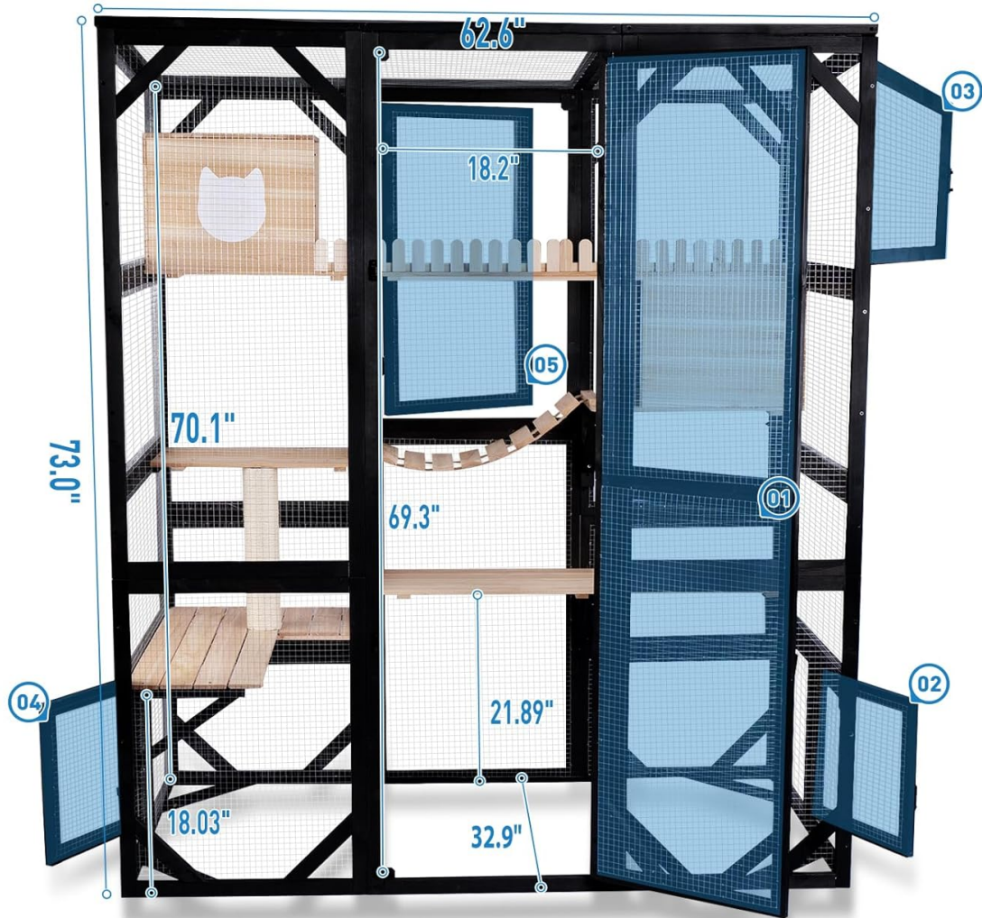
Image 4.1: Catio dimensions and access points for assembly reference.
