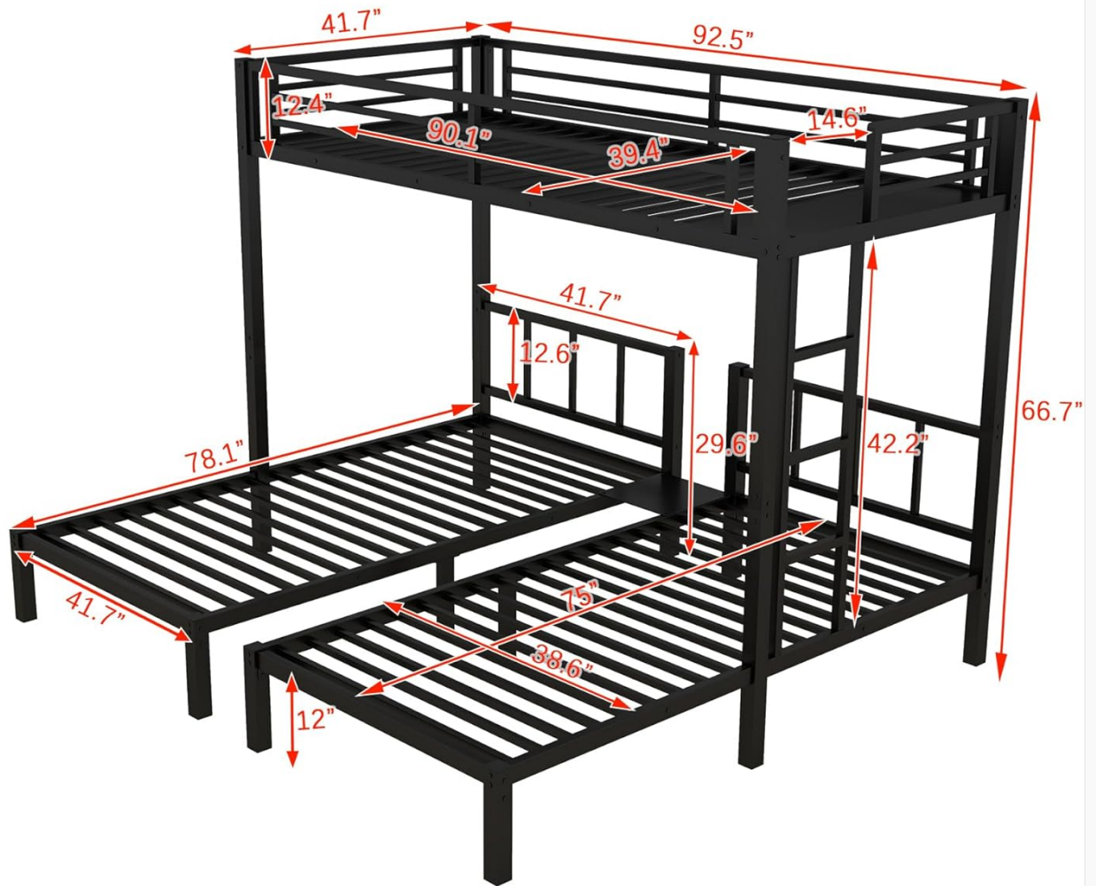
Image 7.1: Dimensional diagram of the Bellemave Triple Bunk Bed.
