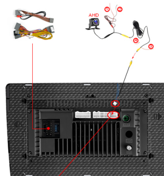
Figure 2: Backup Camera Wiring Diagram. This diagram shows how to connect the backup camera's power and video signal to the car stereo and the vehicle's reversing light circuit. The back wire from the power cable connects to the rear camera. The reversing trigger cable connects to the car's reversing light positive and negative terminals. The white plug must be securely connected to the radio for Bluetooth and Wi-Fi to function.
