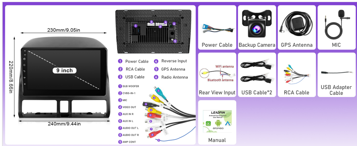
Figure 1: Included components and wiring diagram. This image illustrates the main stereo unit, various connection cables (power, RCA, USB), antennas (GPS, WiFi, Bluetooth, Radio), an external microphone, and the backup camera.
