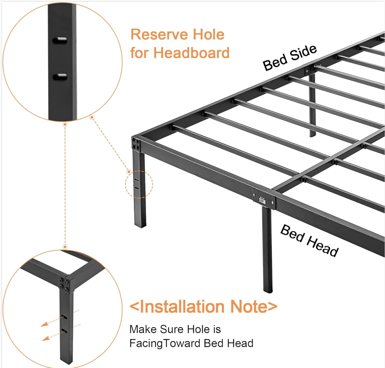
Figure 4.2: Headboard attachment points. This image highlights the pre-drilled holes on the bed frame legs, designed for attaching a headboard. Ensure these holes face the intended head of the bed during assembly.
