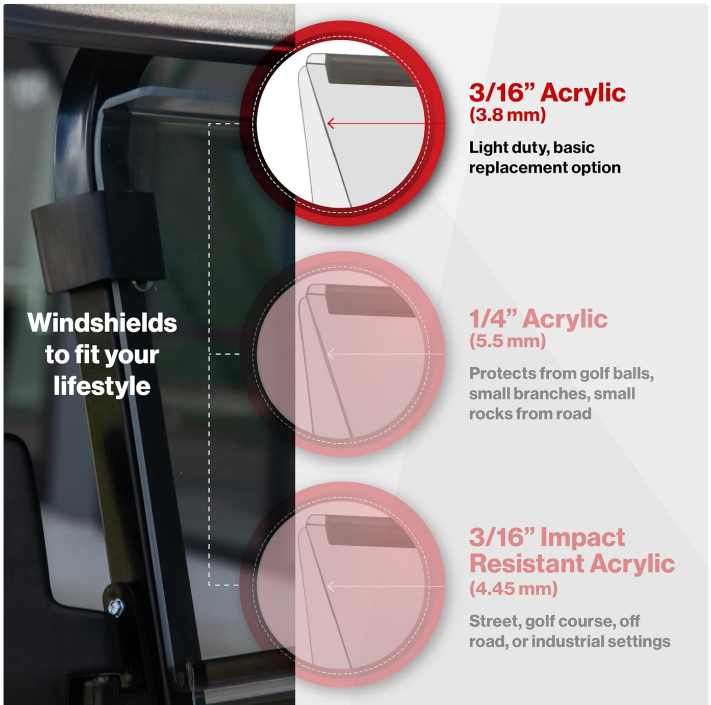
Figure 7.1: Acrylic thickness comparison (this product is 3/16 inch acrylic).
