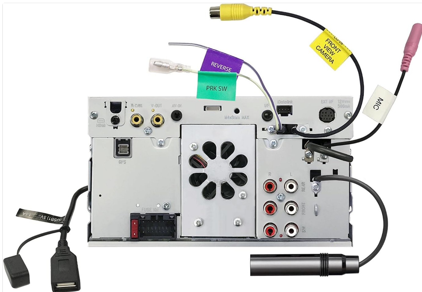
Figure 2: Rear connections of the JVC KW-M780BT Digital Media Receiver.
