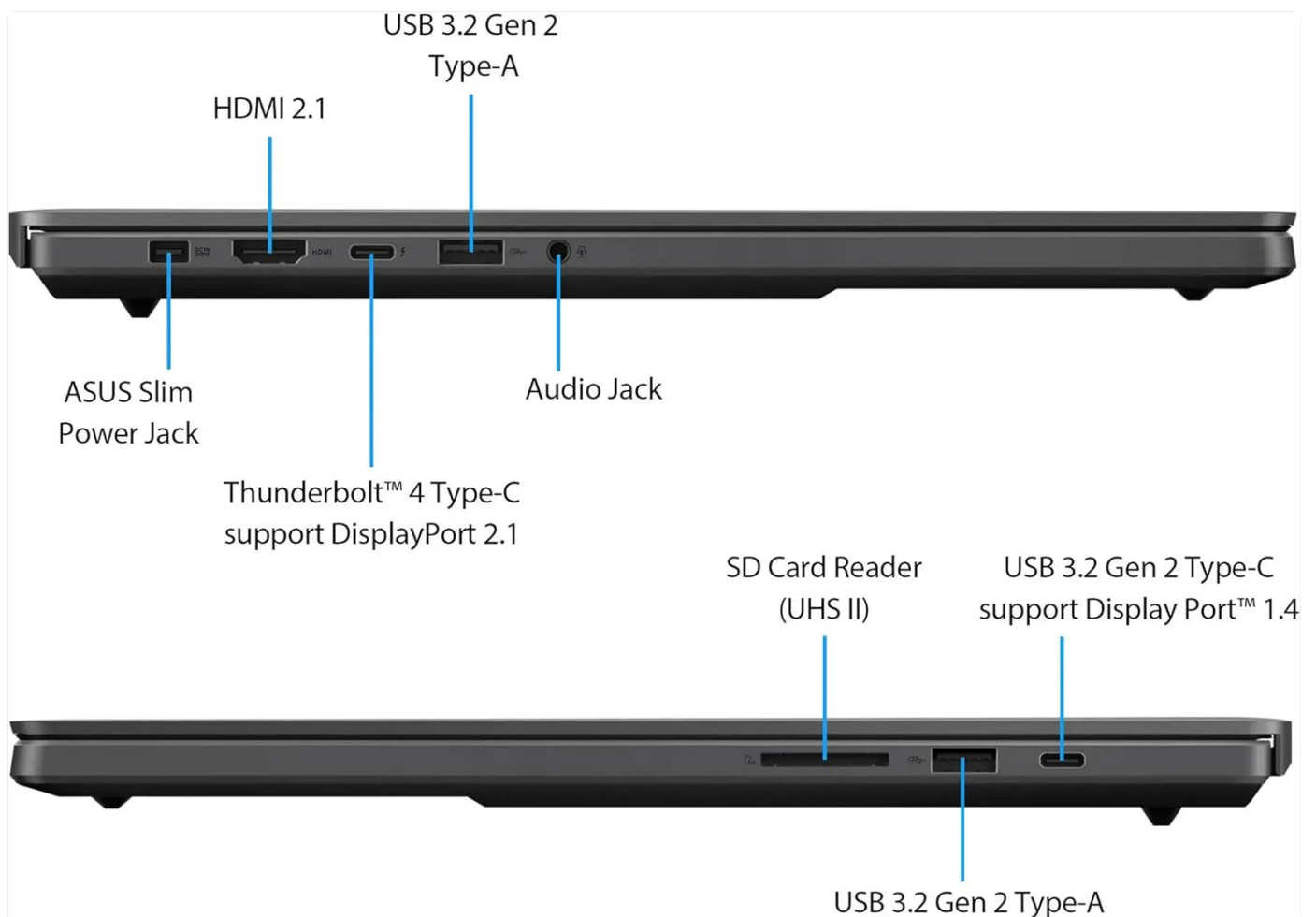
Image: A detailed diagram illustrating the location and type of each port on the laptop's sides.
